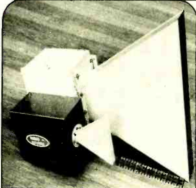
2 GHz & 7 GHz Antenna Elements side by side
