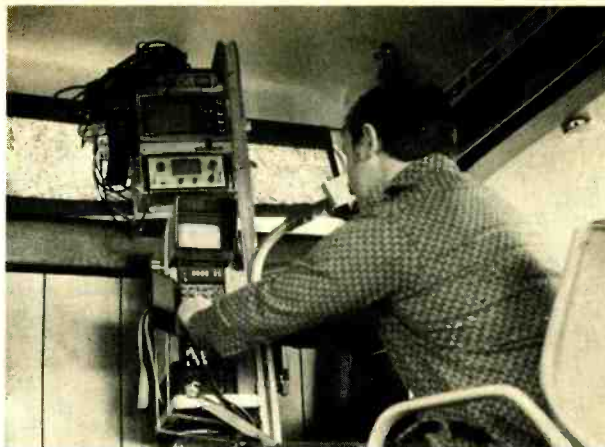
The video cart remains in the van for some taping jobs. Equipment from top to bottom: Shure mixer, five-inch Sony receiver modified as monitor (to verify color), portable Tektronix oscilloscope and waveform monitor, SK-70 backpack with standard viewfinder; Sony 2800 portable recorder; ac power pack for recorder, not shown.
